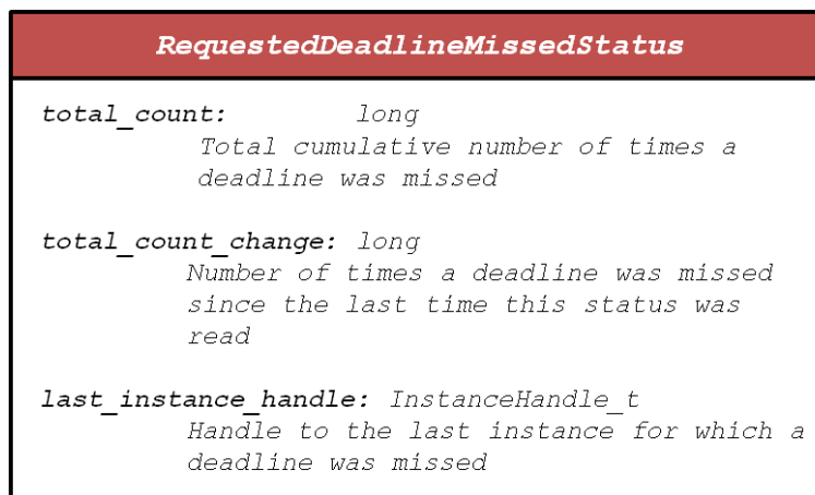
Figure 13-4: Requested Deadline Missed Status Structure
