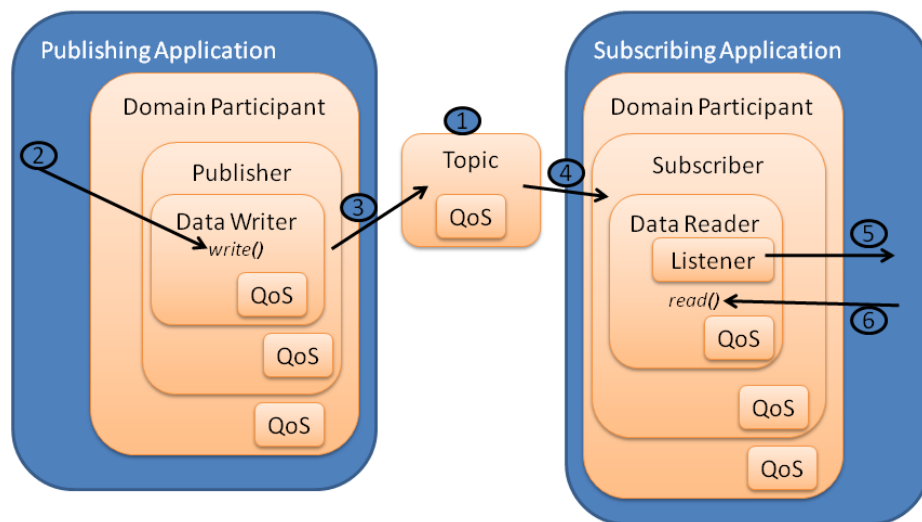
Figure 1-5: DDS Architecture
